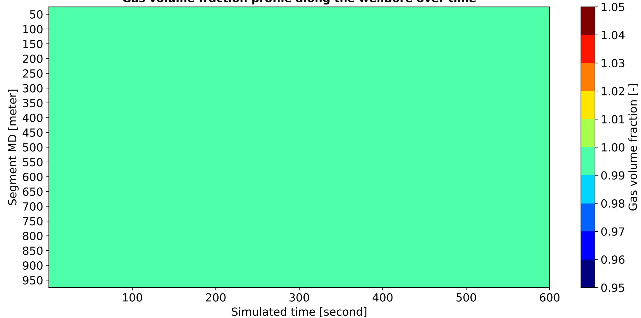
Gas volume fraction profile along the wellbore over time
